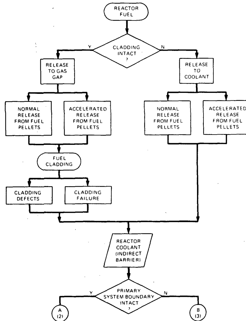
Figure D.2. Pathways for release of radionuclides in liquid stream from a BWR during ATWS.
