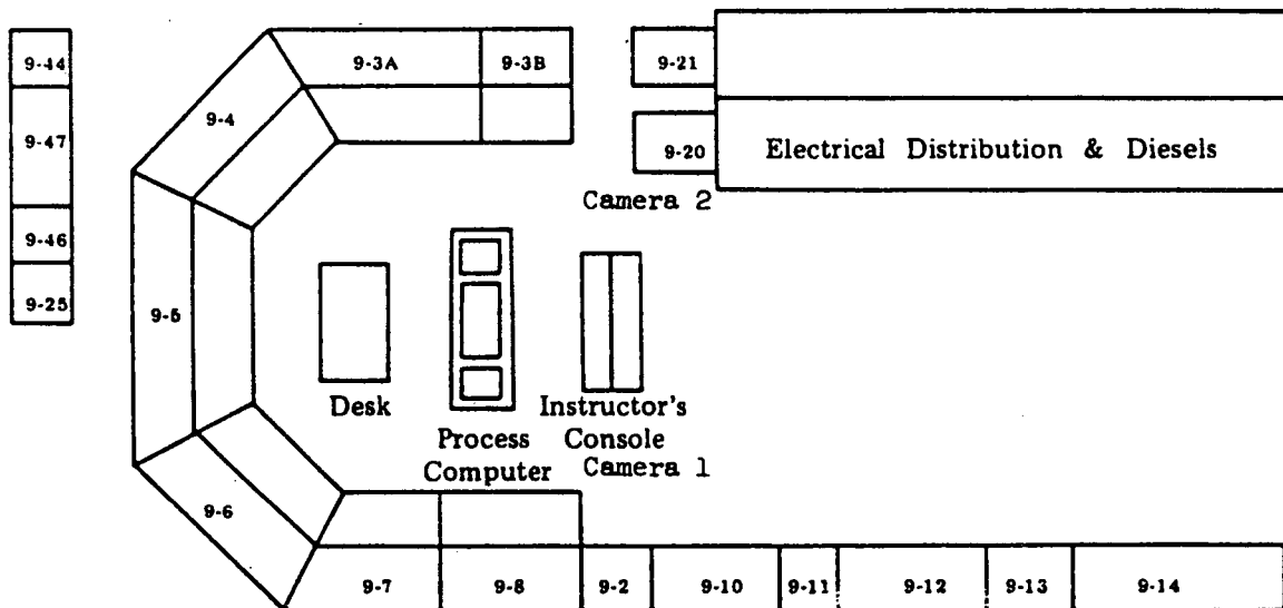
Simulator Control Room Layout
