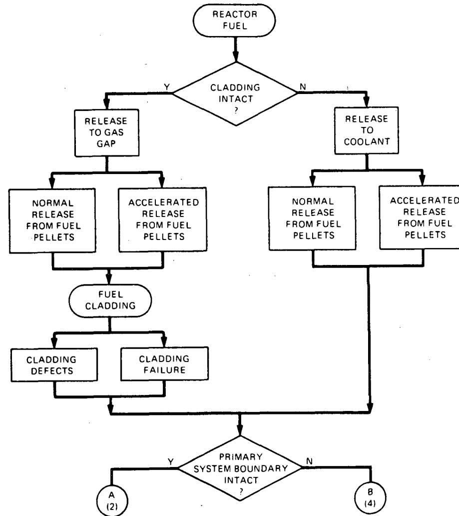
Figure D.1. Pathways for the release of gaseous and airborne particulate radionuclides from a BWR during ATWS.
