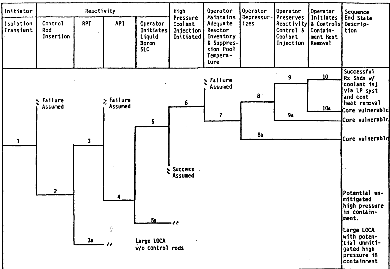
Figure 2.2. Operator action event tree for ATWS initiated by closure of main steam isolation valves (from Ref. 13).
